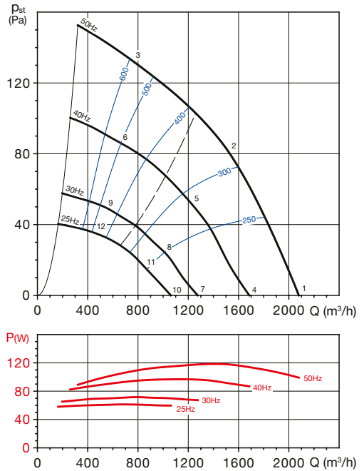
CRVT/6-355 N
