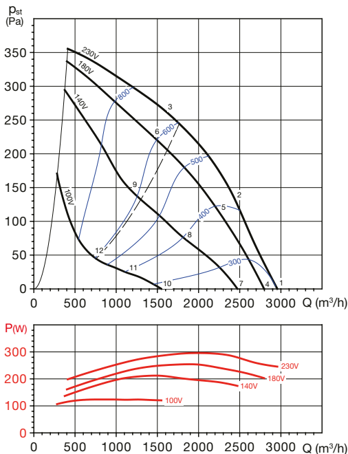
CRVB/4-355 N
