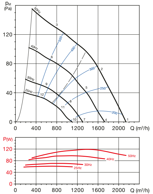
CRHT/6-355 N
