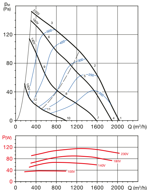
CRVB/6-355 N
