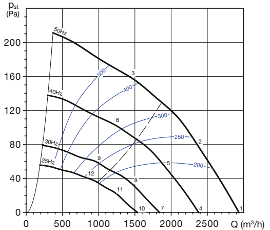
CRHT/6-400 N
