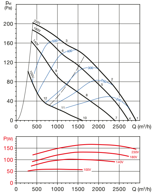
CRVB/6-400 N
