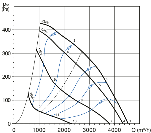
CRHB/4-400 N
