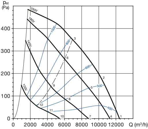
CRVB/6-630 N
