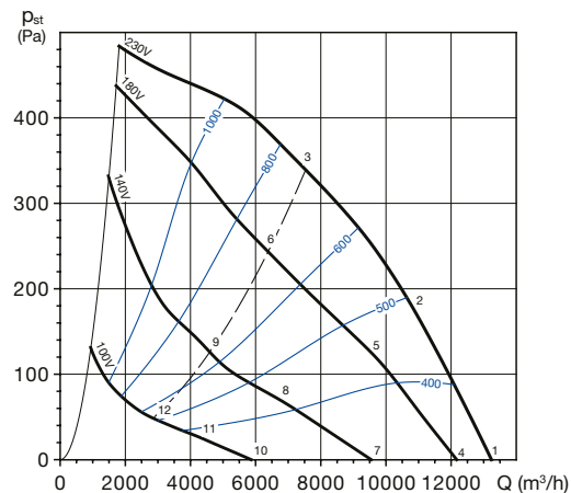
CRHB/6-630 N
