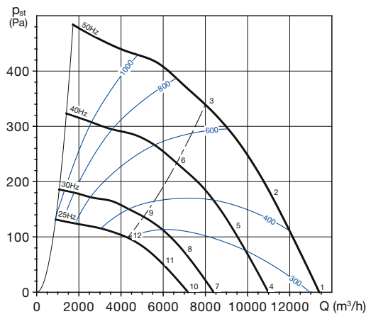
CRHT/6-630 N
